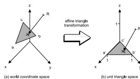
Figure 1: The unit triangle intersection method consists of two stages: First the ray is transformed, using a triangle specific affine triangle transformation. In the second stage, a simple intersection test of the transformed ray with the unit triangle is performed.
